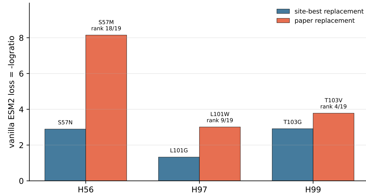
B. Vanilla MULTI-evolve zero-shot
