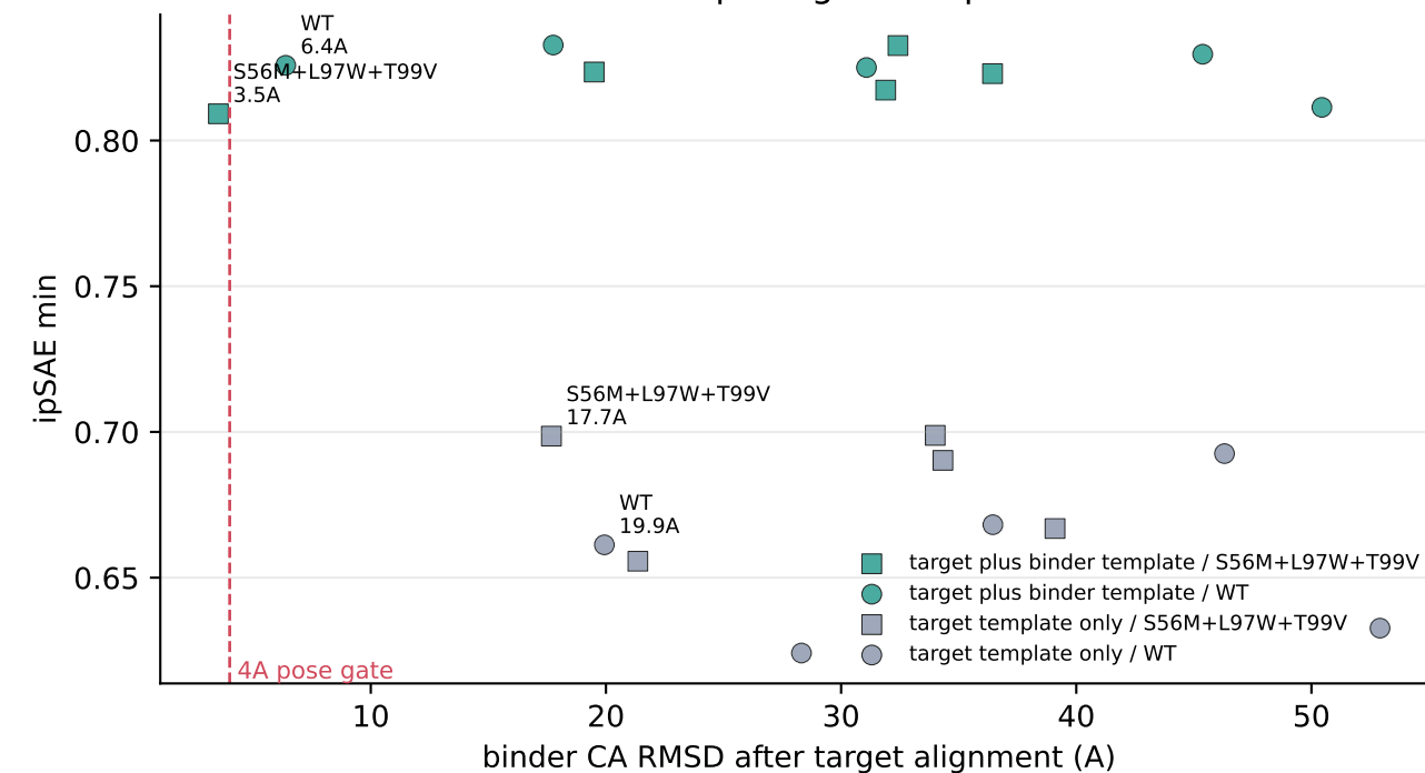
D. Refold pose gate vs ipSAE
